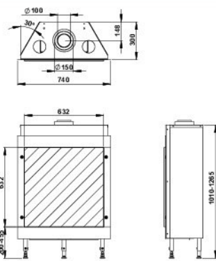
Trimline 63 H DB
