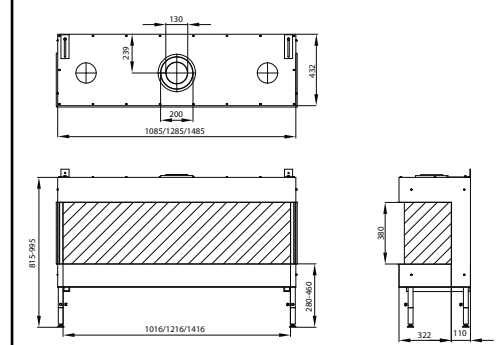
Trimline 100 / 120 / 140 Panorama DB
