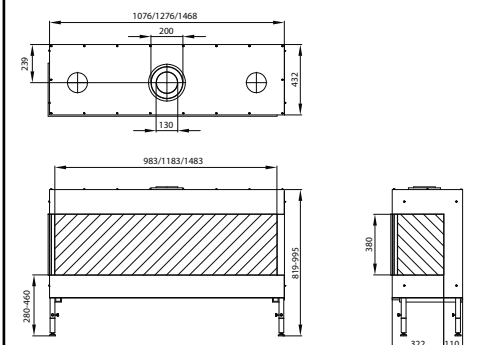
Trimline 100 / 120 / 140 Corner DB
