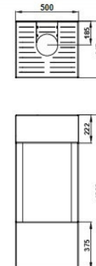
Trimline 38 FS Mantel
