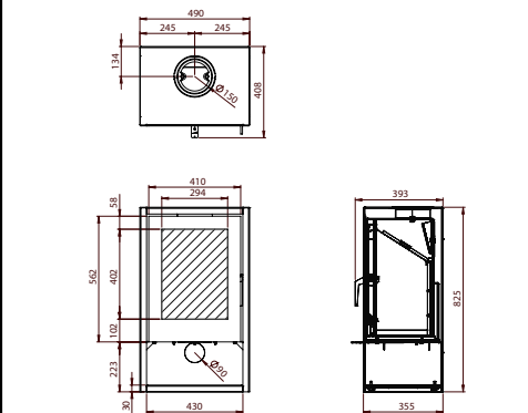
Woodfire Cubic 6kW
