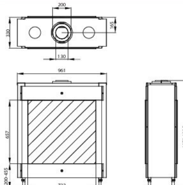
Trimline 73 Tunnel DB
