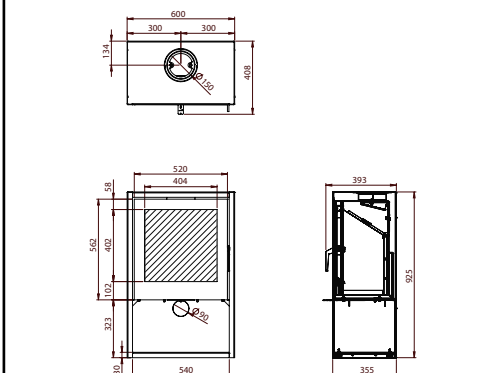
Woodfire Cubic 8kW
