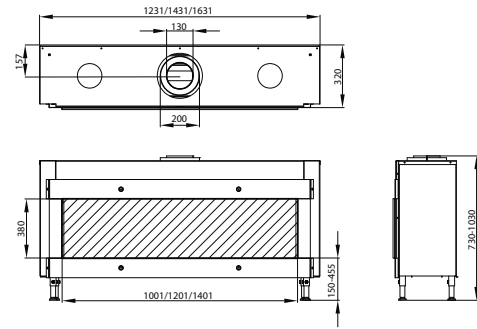
Trimline 100 / 120 / 140 Front DB
