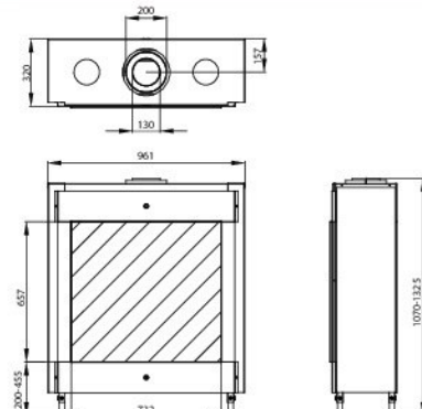
Trimline 73 H DB
