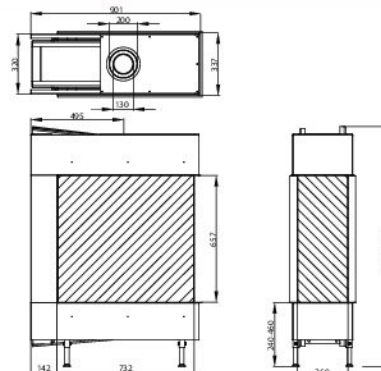
Trimline 73 Room divider DB
