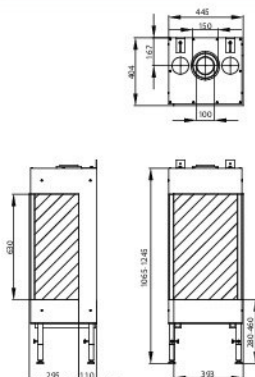
Trimline 38 Corner (right)
