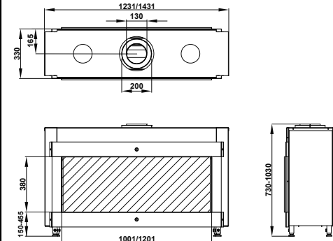
Trimline 100 / 120 Tunnel DB
